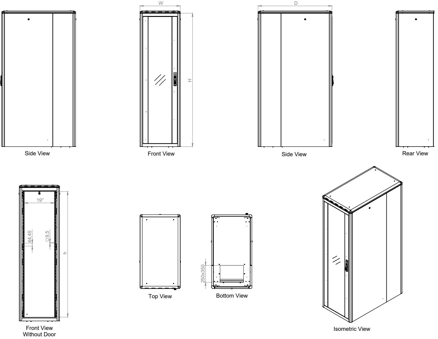
19" Ager Vega Dikili Tip Kabineler W=600mm D=1100mm
