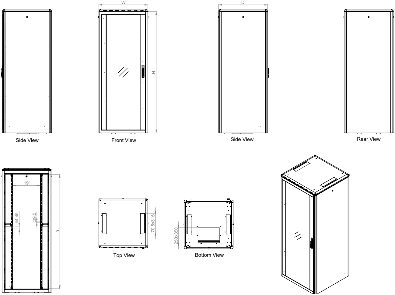
19" Ager Vega Dikili Tip Kabineler W=800mm D=800mm
