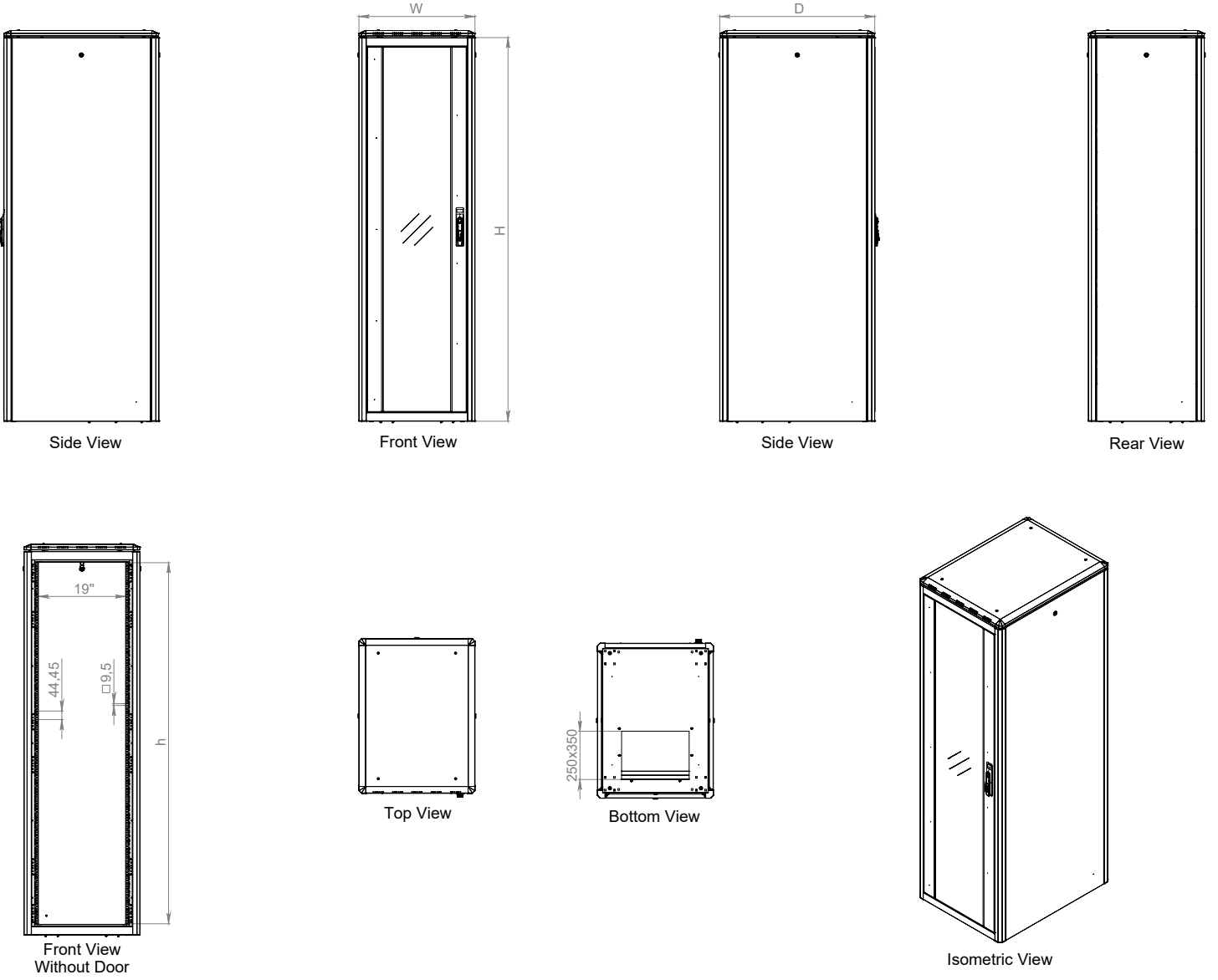
19" Ager Vega Dikili Tip Kabinetler W=600mm D=800mm
