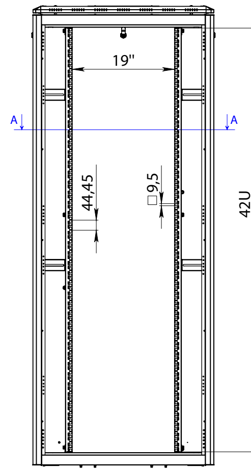
FRONT VIEW WITHOUT DOORS
