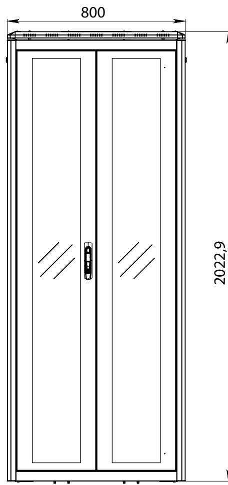
FRONT VIEW
