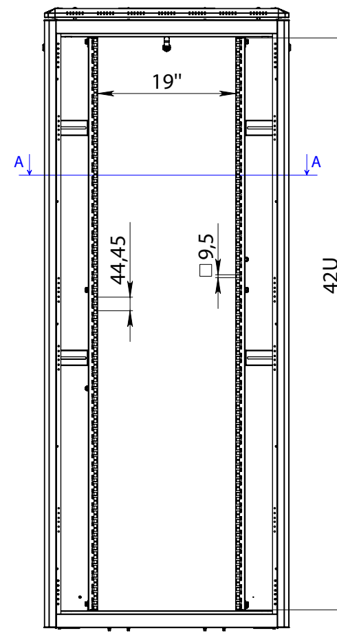
FRONT VIEW WITHOUT DOORS
