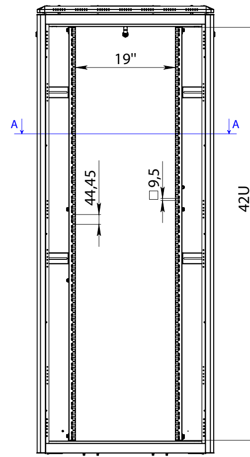
FRONT VIEW WITHOUT DOORS
