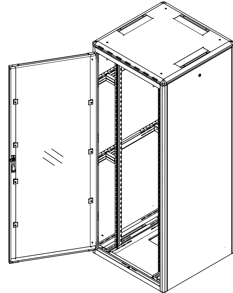
ISOMETRIC VIEW
