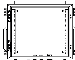
Front View Without Door
