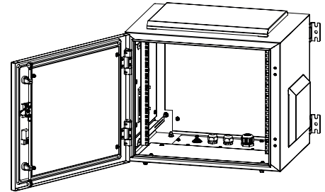
Isometric View Without Door
