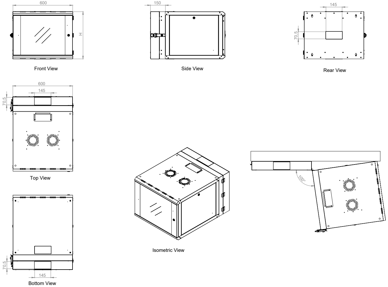
19" Ager Wall Mounted AGENA Double Section Series
