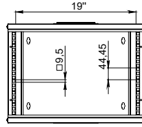
FRONT VIEW WITHOUT DOOR
