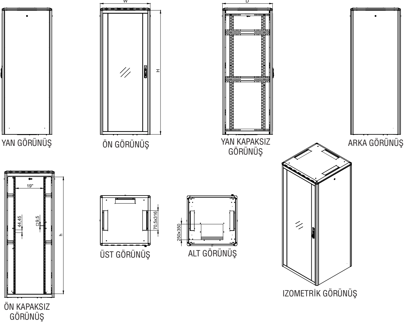
19" Ager Vega Dikili Tip Kabinetler W=800mm D=800mm
