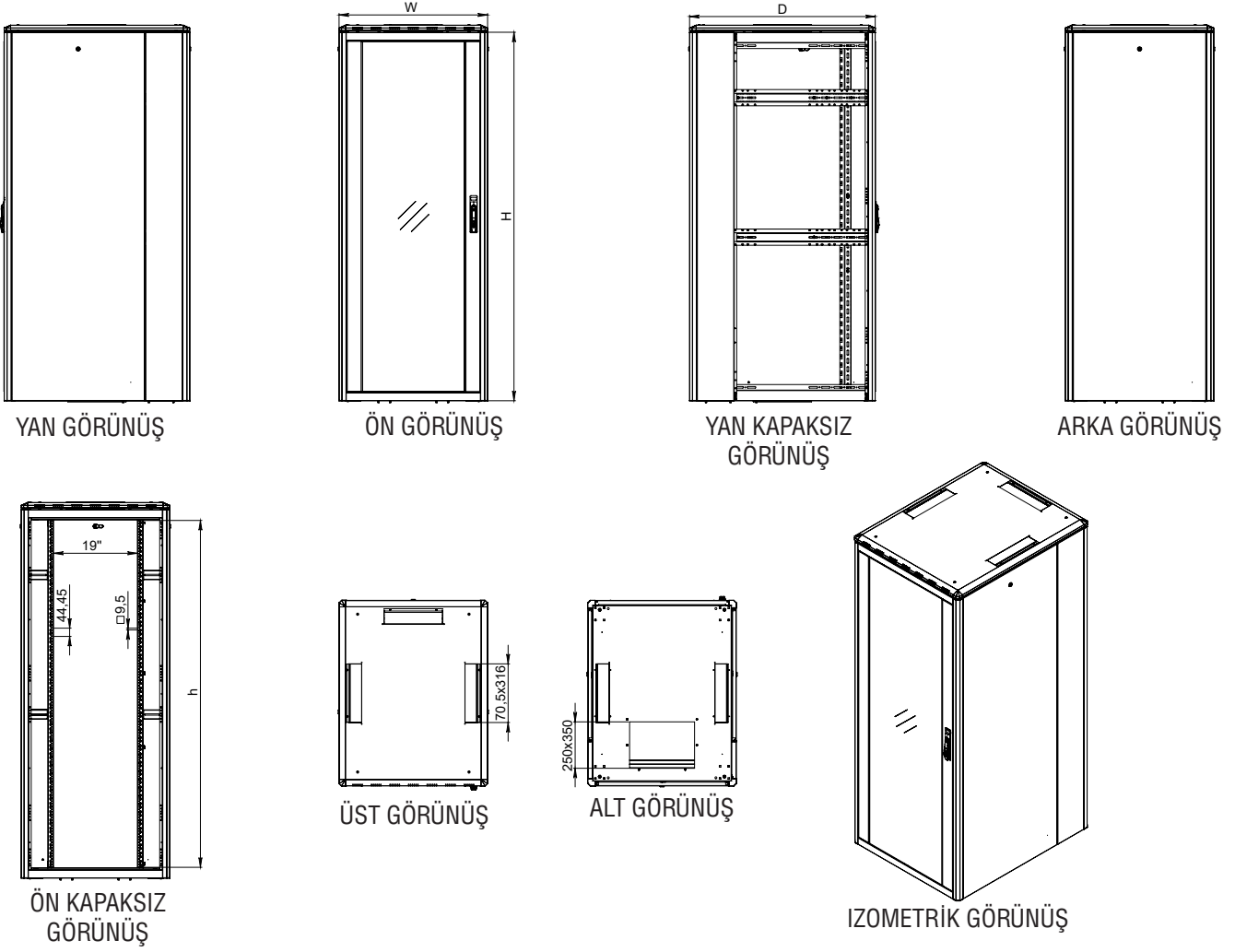
19" Ager Vega Dikili Tip Kabinetler W=800mm D=1000mm
