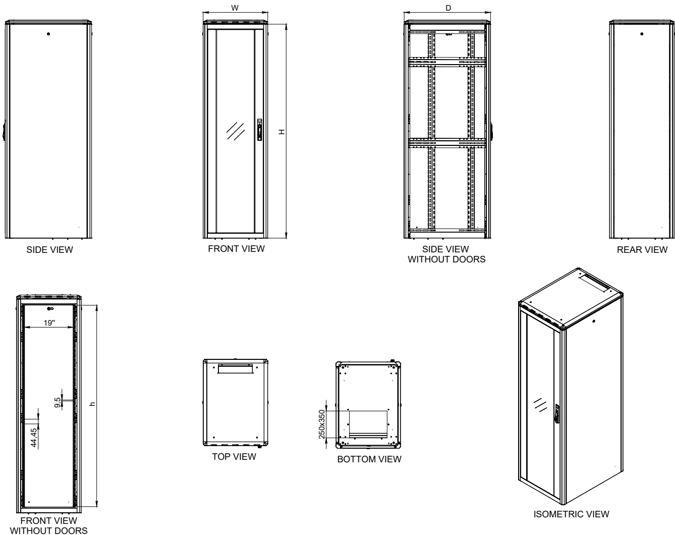
19" Ager Vega Free Standing Cabinets W=600mm D=800mm
