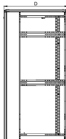
SIDE VIEW WITHOUT DOORS
