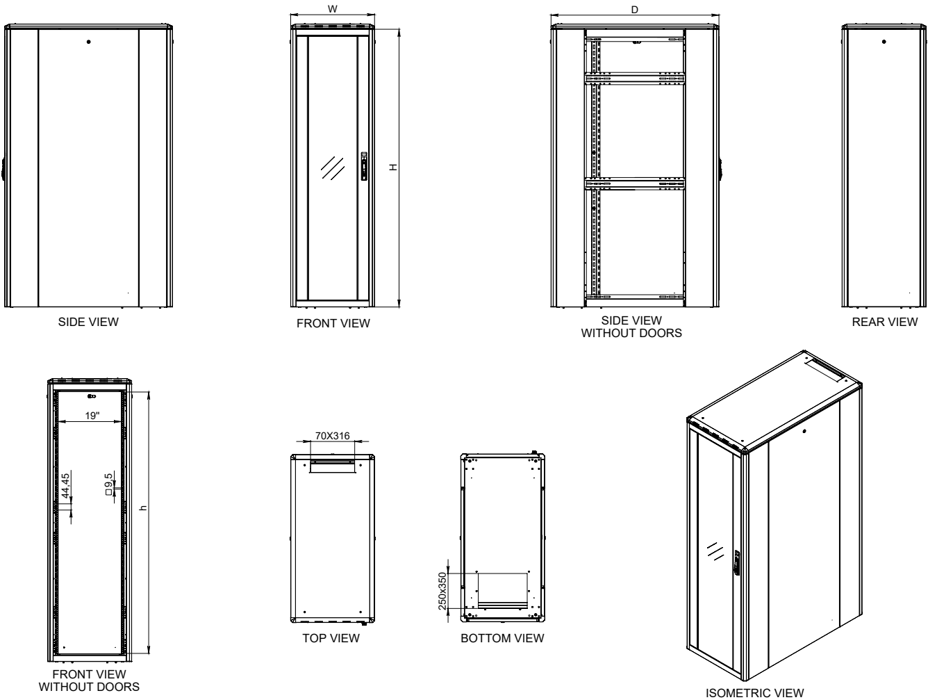
19" Ager Vega Free Standing Cabinets W=600mm D=1200mm
