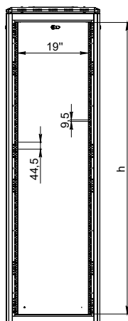
FRONT VIEW WITHOUT DOORS
