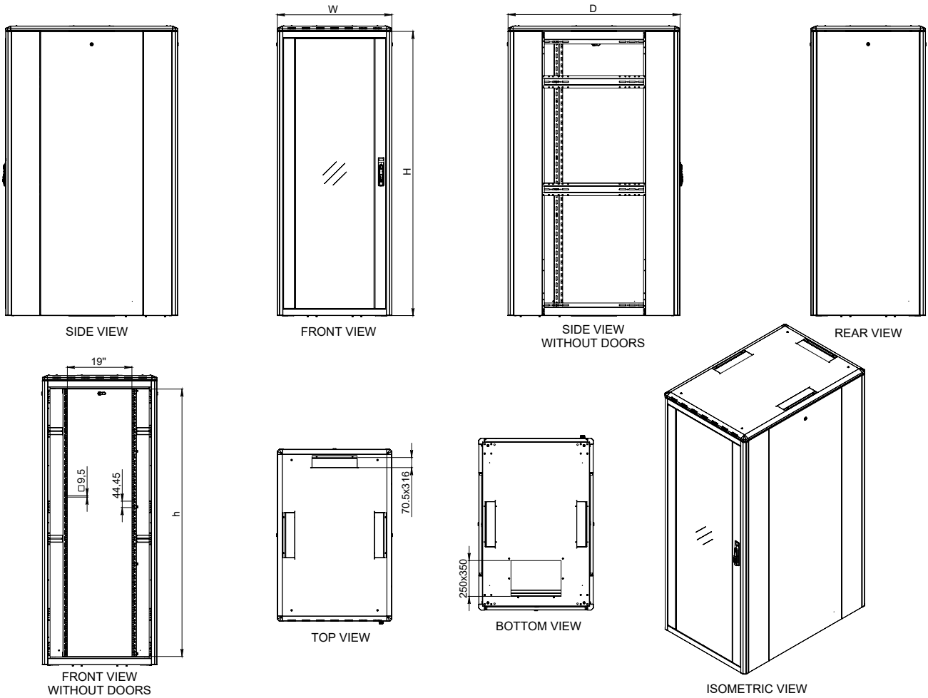
19" Ager Vega Free Standing Cabinets W=800mm D=1200mm
