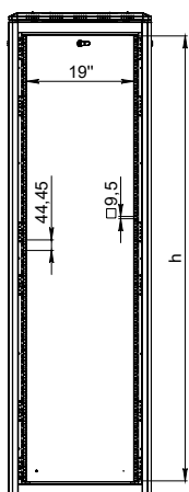
FRONT VIEW WITHOUT DOORS
