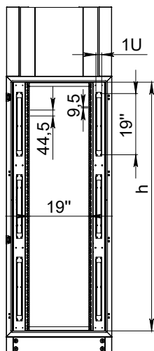
FRONT VIEW WITHOUT DOORS
