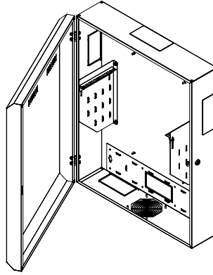
ISO VIEW/DOOR OPEN
