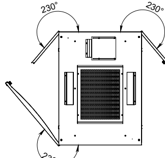
DOOR OPENING ANGLE
