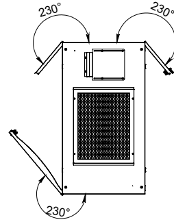
DOOR OPENING ANGLE
