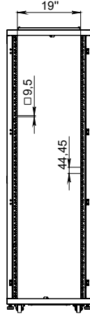
FRONT VIEW WITHOUT DOOR
