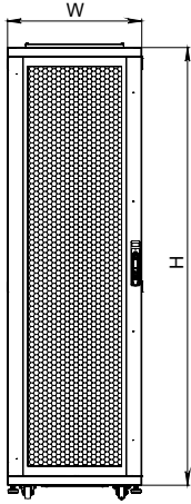
FRONT VIEW
