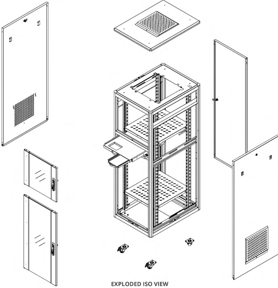
EXPLODED ISO VIEW
