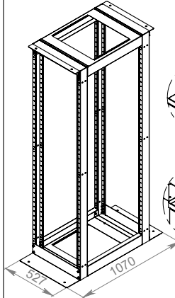
Isometric View D:1070 mm
