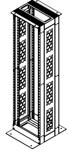
52 mm sized honeycomb Side panel for airflow
