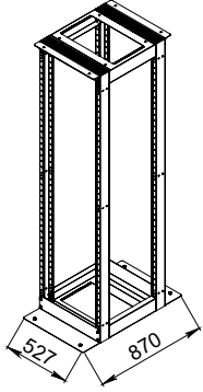
Isometric View D:870 mm
