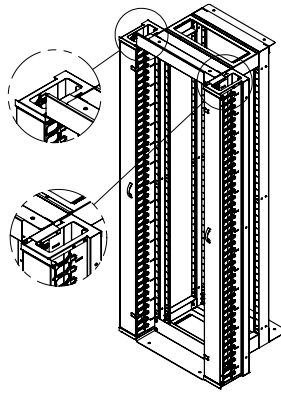
W:135 mm Finger Cable Management
