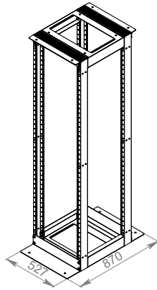
Isometric View D:870 mm
