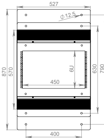
Top View D:870 mm
