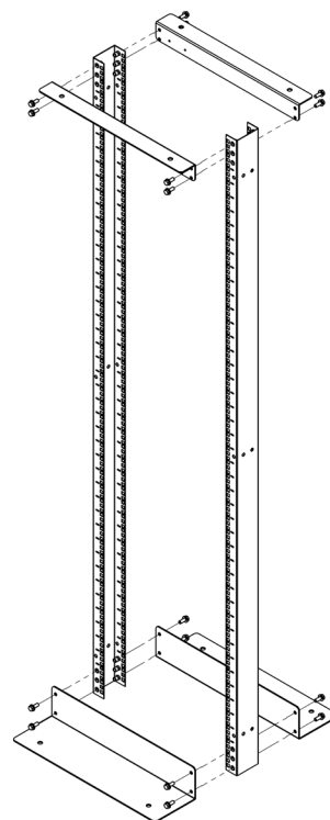
Exploded View
