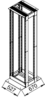
Isometric View D:670 mm
