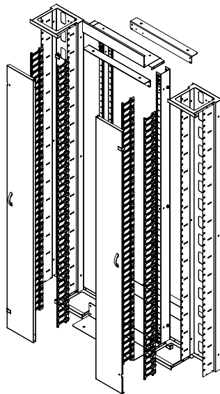
EXPLODED VIEW
