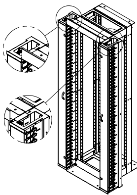
W:135 mm Finger Cable Management
