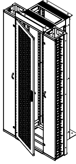
%63 Perforated Front/Rear door application
