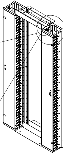
ISOMETRIC VIEW
