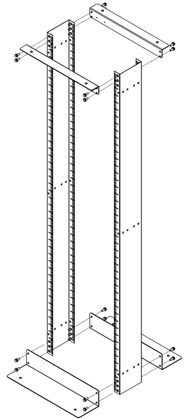
Exploded View
