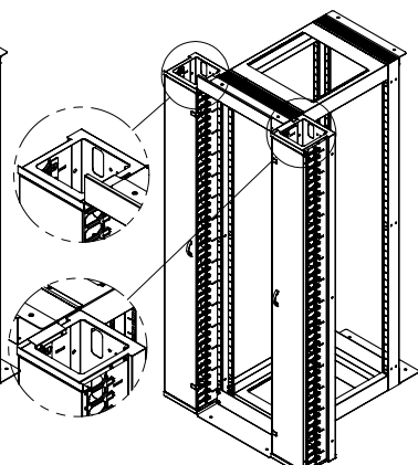
W:235 mm Finger Cable Management
