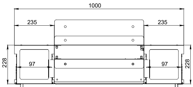
TOP VIEW DIMENSIONS
