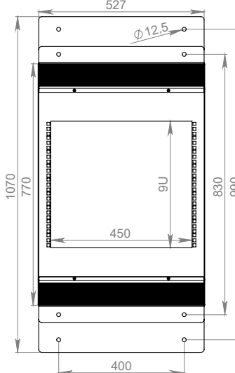
Top View D:1070 mm
