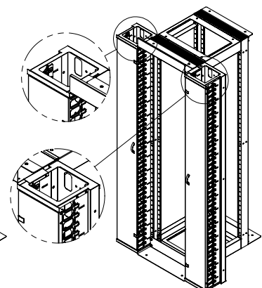
W:235 mm Finger Cable Management
