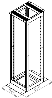
Isometric View D:870 mm
