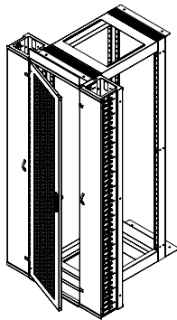
%63 Perforated Front/Rear door application
