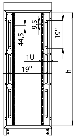
FRONT VIEW WITHOUT DOORS
