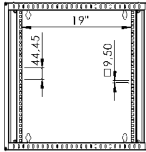
Front View Without Door
