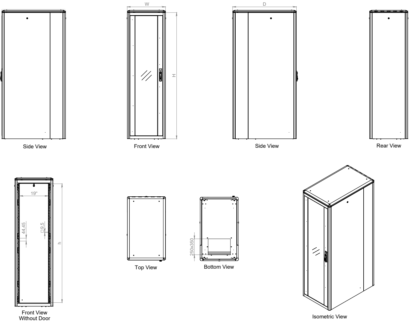
19" Ager Vega Free Standing Cabinets W=600mm D=1000mm
