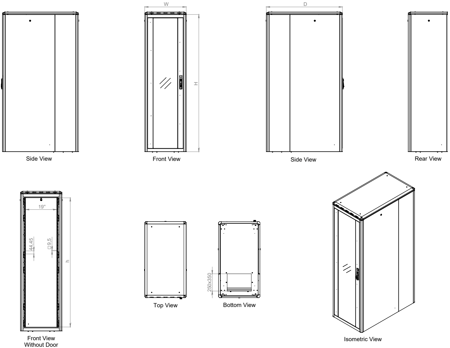
19" Ager Vega Free Standing Cabinets W=600mm D=1100mm
