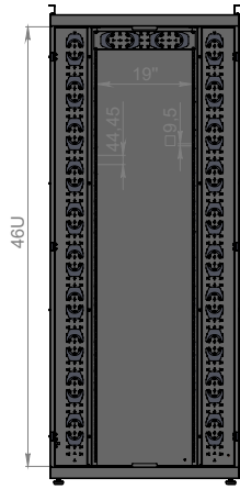
Inside View
